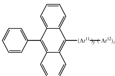
[Chemical Formula 2]
