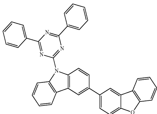
[Chemical Formula 7]
