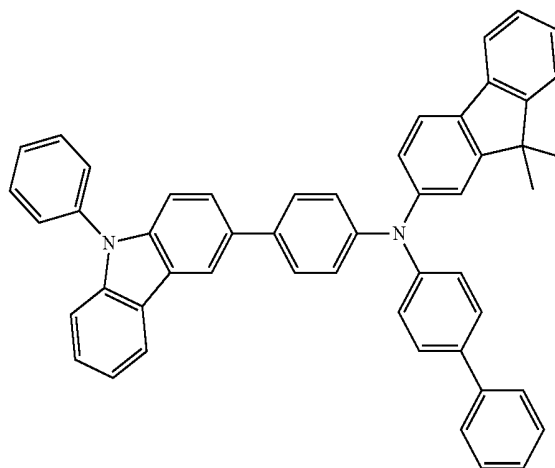
[Chemical Formula 5]
