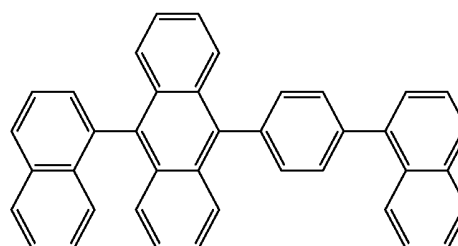
[Chemical Formula 8]
