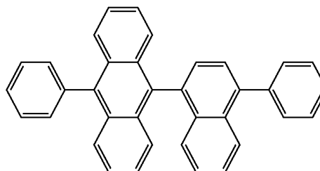
[Chemical Formula 2-1]
