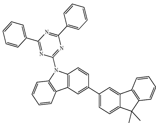
[Chemical Formula 6]
