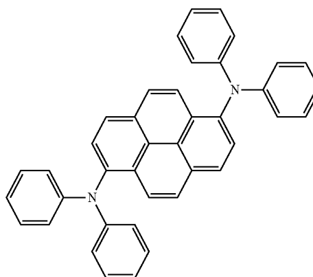
[Chemical Formula 3]
