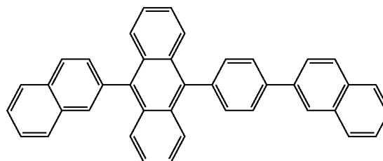
[Chemical Formula 8]
