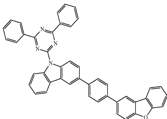
[Chemical Formula 8]
