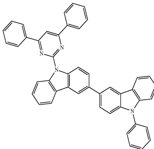
[Chemical Formula 2]
